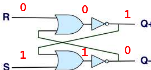
置1 Setting
