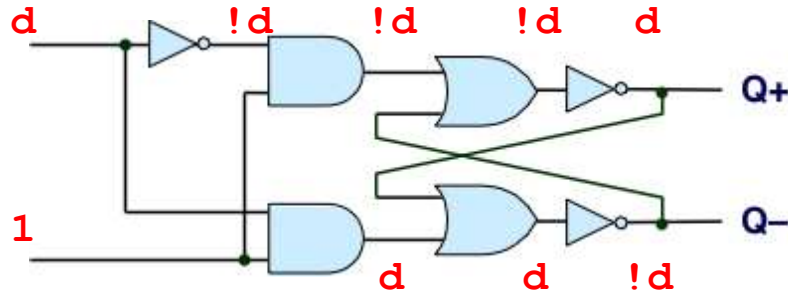
锁定 Latching
